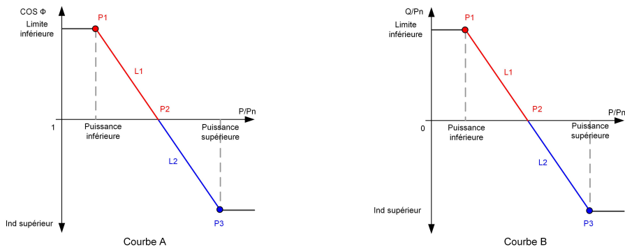
figure 8-3 Courbe Q(P)
