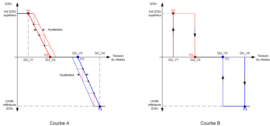
figure 8-4 Courbe Q(U)
