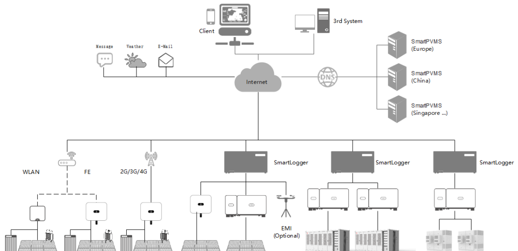
Figure 5-2 SmartPVMS components
