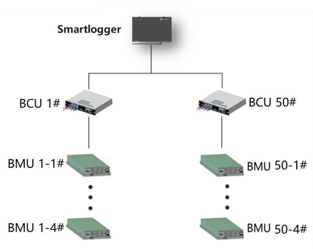
Figure 3-4 Monitoring unit networking diagram
