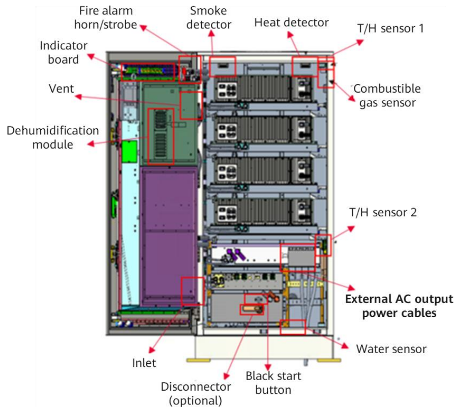
Figure 3-3 ESS interior
