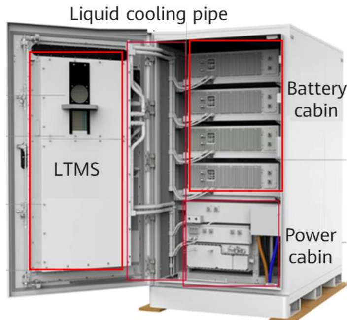
Figure 3-5 Embedded LTMS
