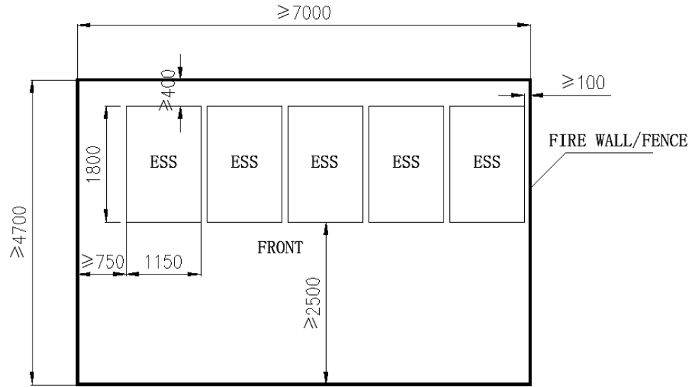
Figure 4-4 Typical array layout (0.75 MWh) (single-row layout)
