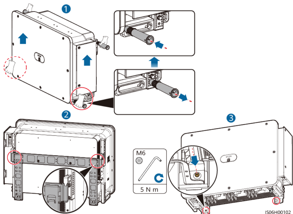
Figure 4-13 Installation
